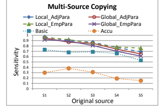
Figure 10: Multi-source copying.
