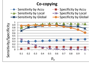
Figure 9: Co-copying.
