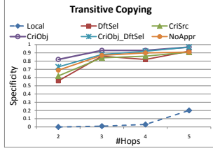
Figure 8: Specificity vs. #hops.
