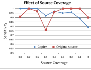
Figure 12: Effect of source coverage.
