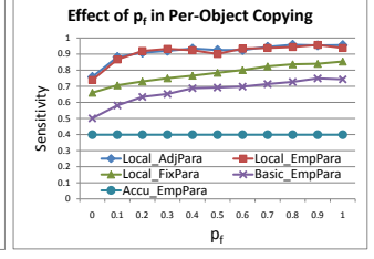
Figure 14: Effect of format keeping rate.
