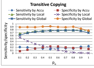
Figure 7: Transitive copying.
