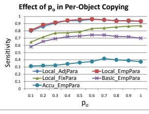
Figure 13: Effect of object selectivity.
